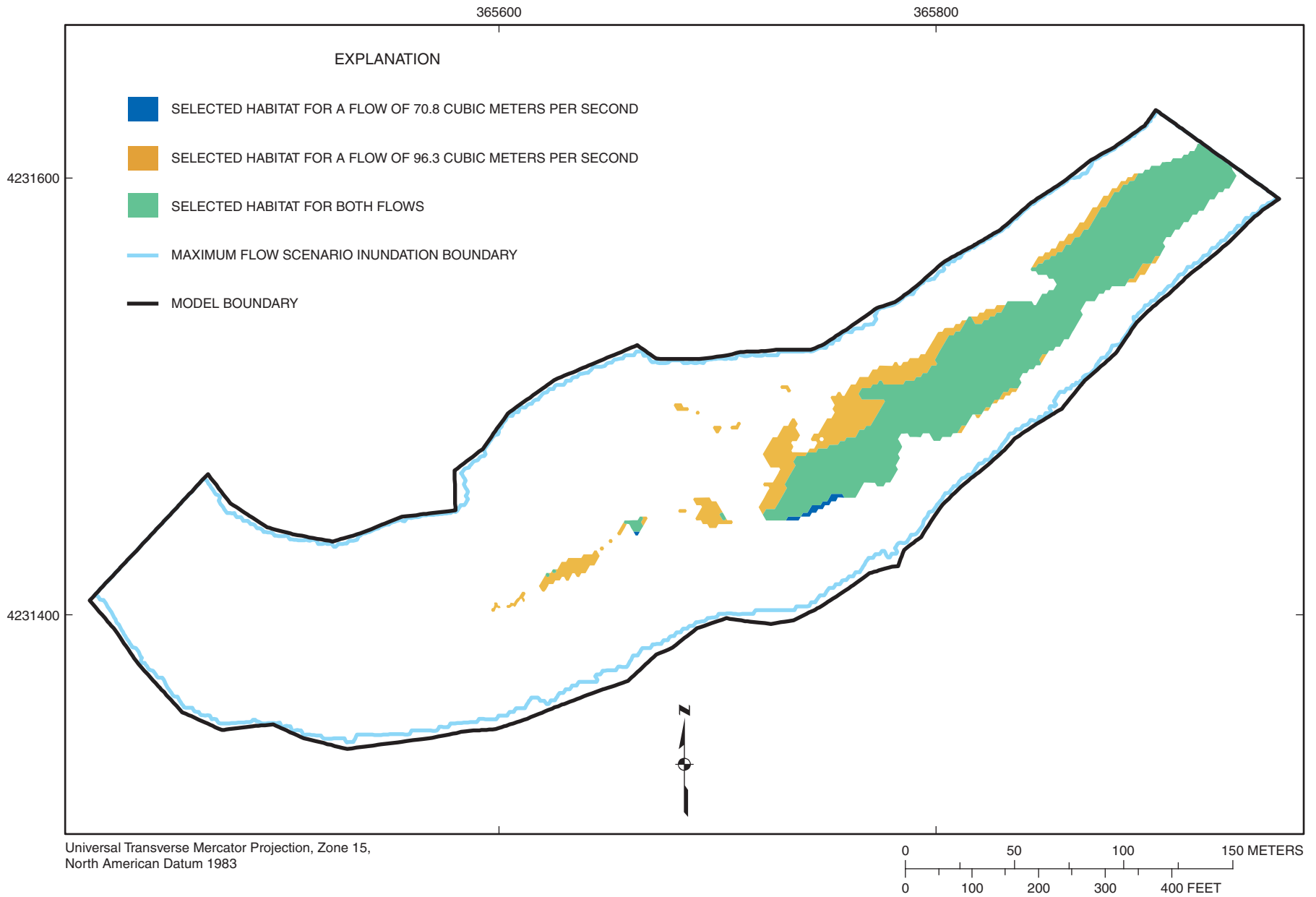
Figure 4-27. Selected habitat area distribution for habitat category 7 (paddlefish) at flows of 70.8 and 96.3 cubic meters per second at Marais des Cygnes River site MDC2.
